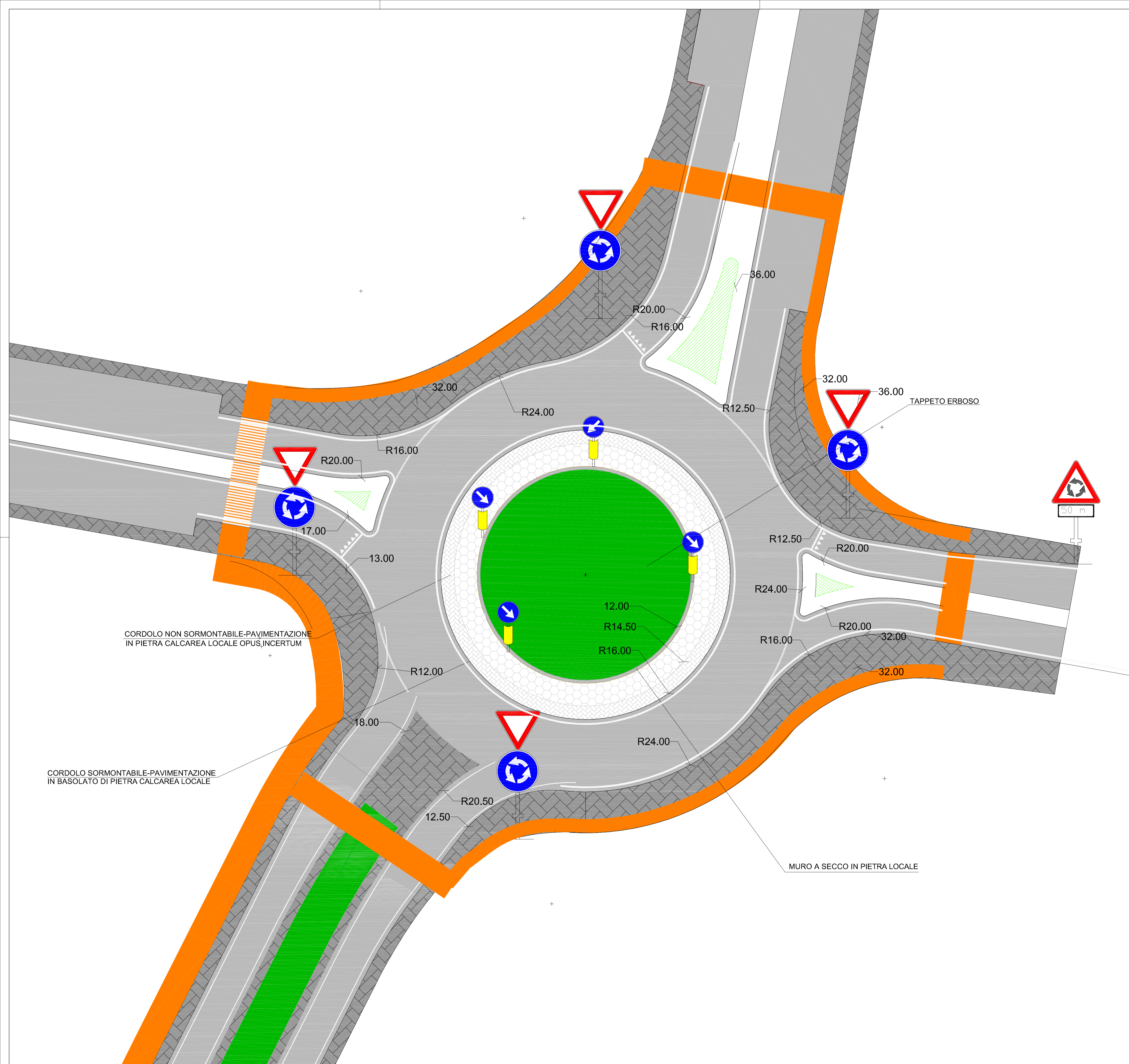
KEY PLAN
