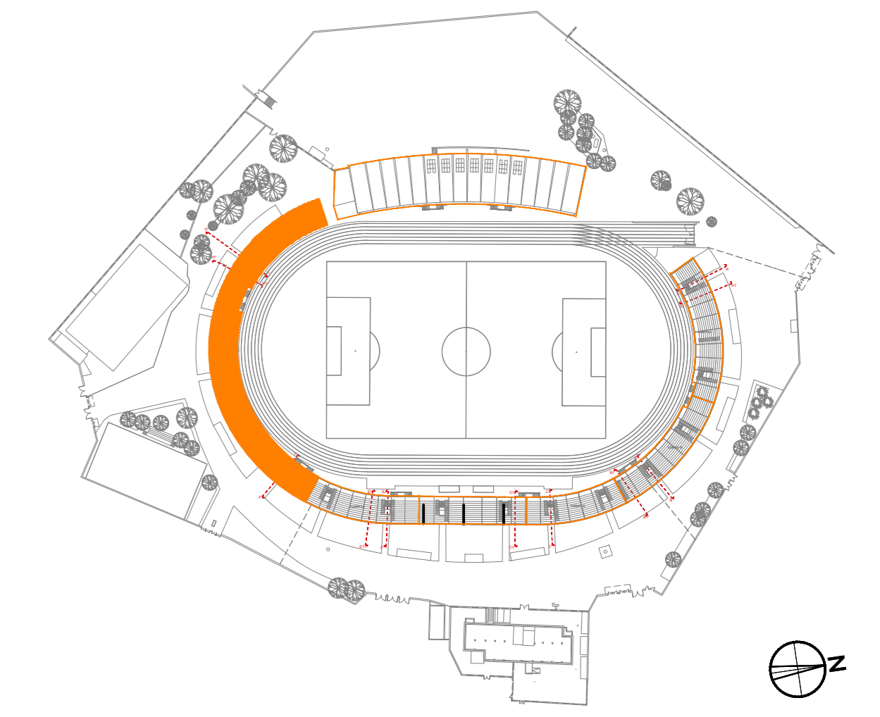
KEY PLAN
