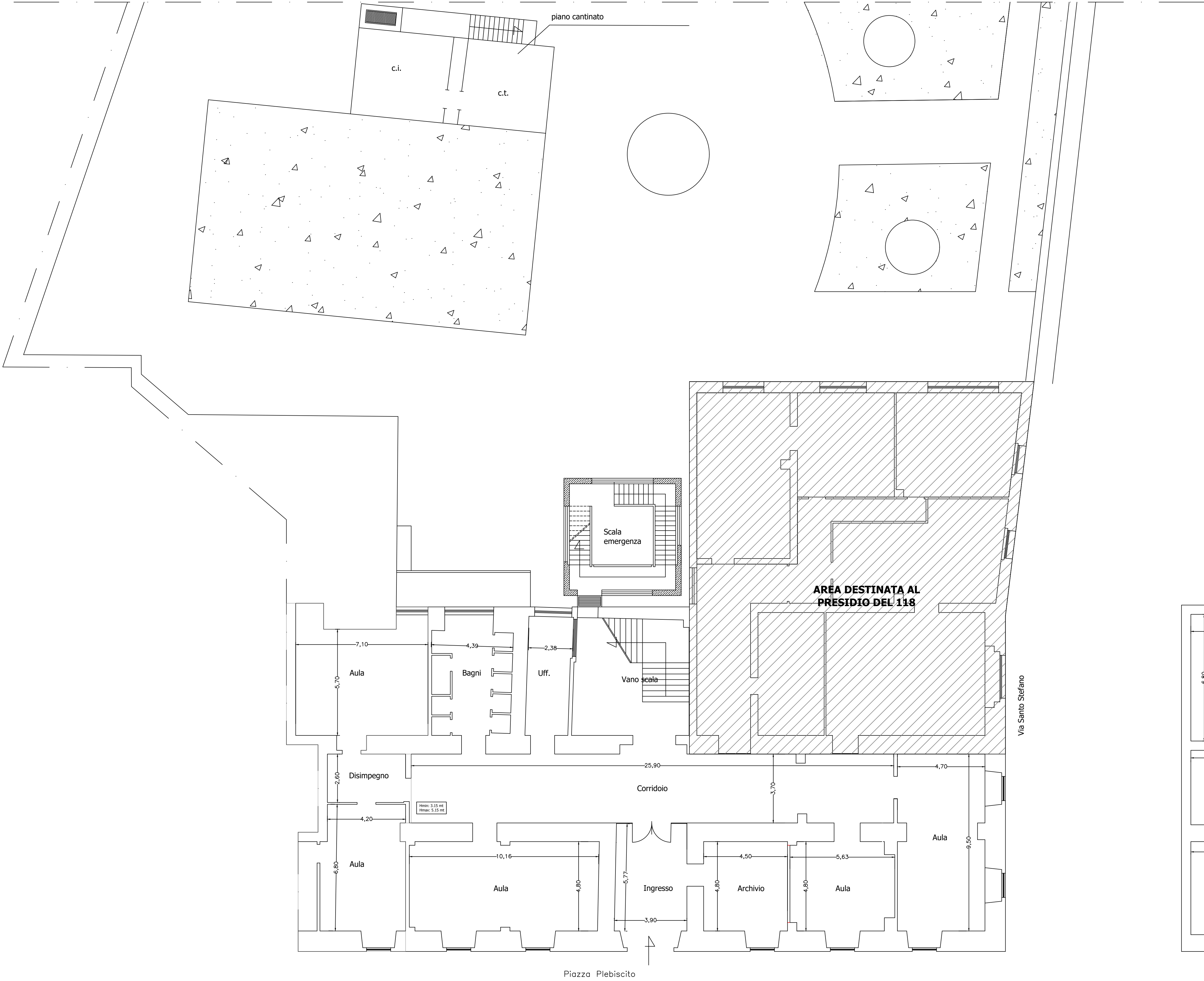
PLANIMETRIA PIANO TERRA
