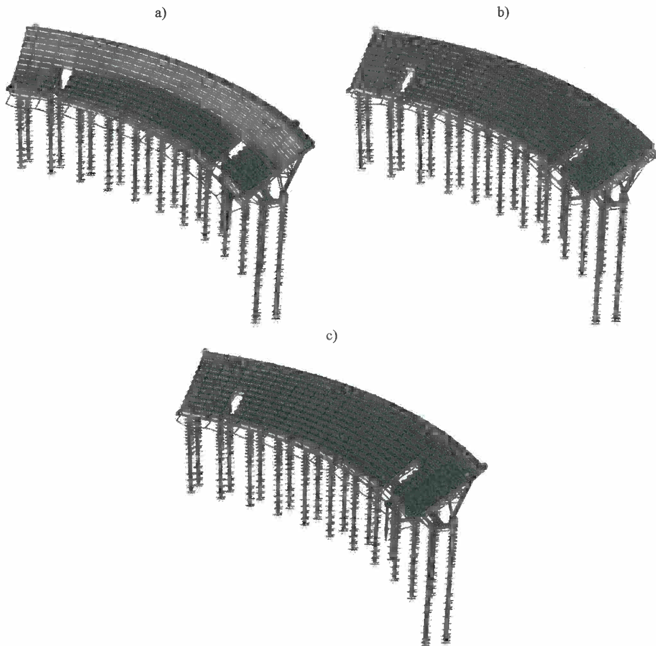
Figura 2 Deformate Corpo A: a) Comb. 100%Ex+30%Ey; b) Comb. 30%Ex+100%Ey; c) Comb.Rara.
